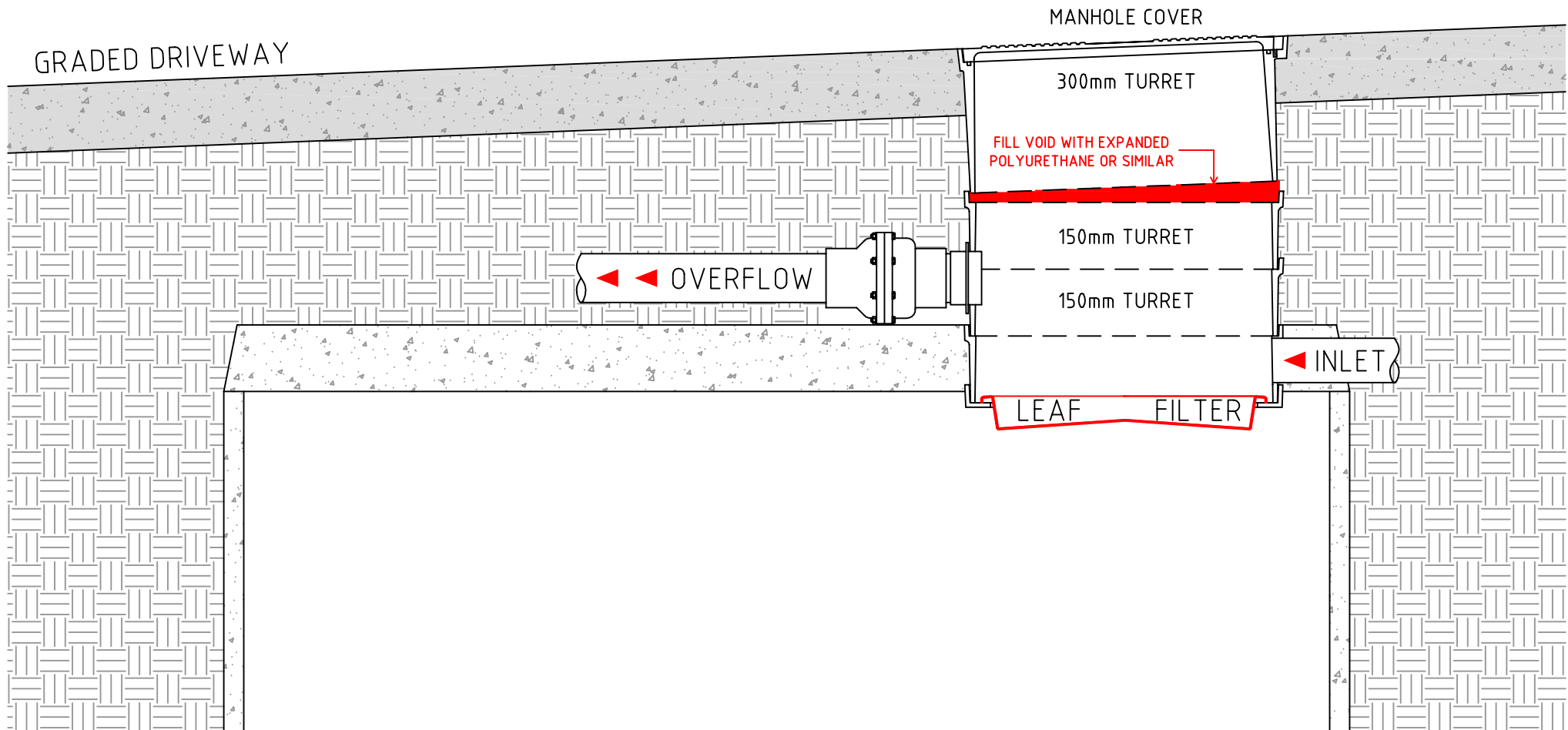
DIAGRAMMATIC SECTION DETAIL
