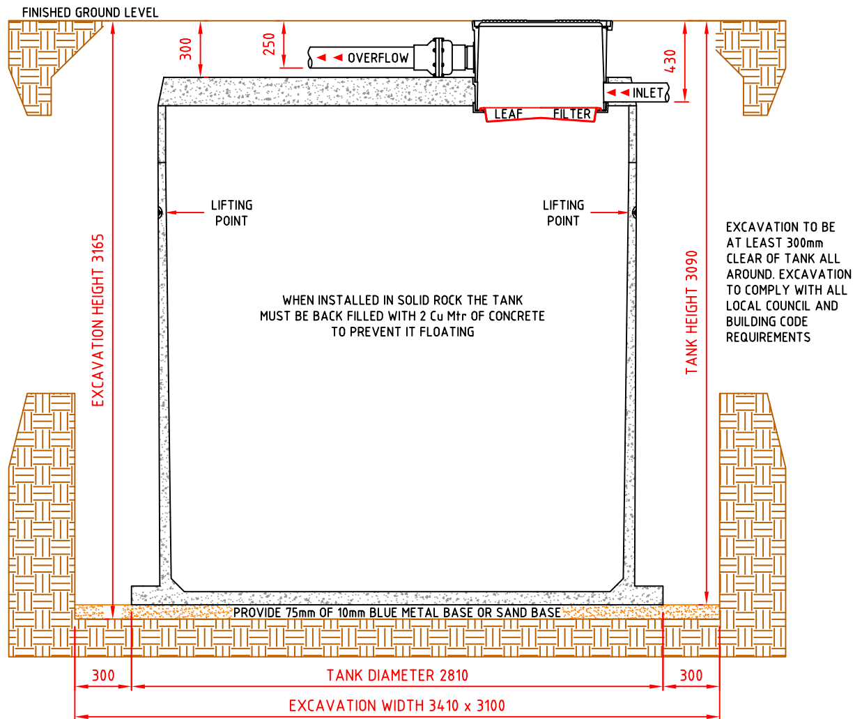
DIAGRAMMATIC SECTION DETAIL
